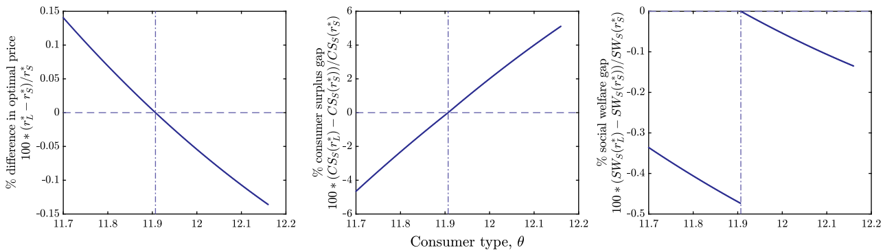
Figure 8. (Color online) Plot of the Percentage Consumer Surplus Gap and Percentage Social Welfare Gap Resulting from Mispriicing Shift Workers as Gig Workers Against Consumer Type \theta
