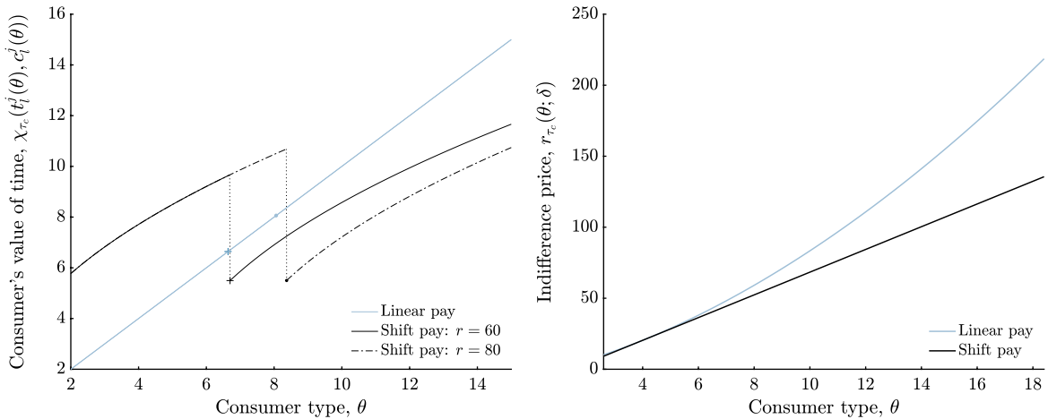
Figure 1. (Color online) Numerical Demonstration of the Consumer's Value of Time (Left), \chi_{\tau_c}(t_l^j, c_l^j) and the Indifference Price r_{\tau_c}(\theta; \delta) of Consumers Paid Under Linear and Shift Pay Compensation Structures
